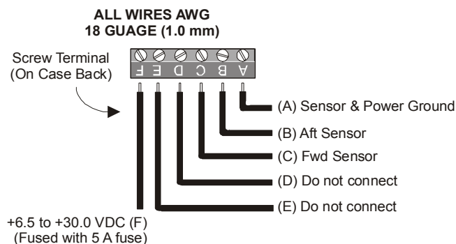
Figure 4 - Wiring Diagram
